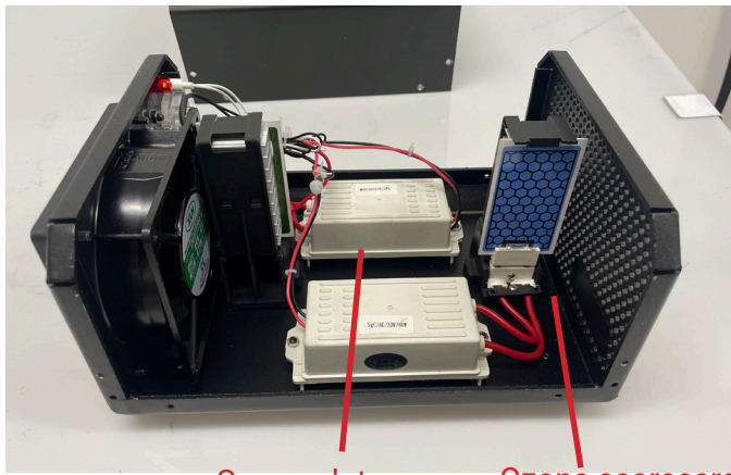
Ozone plate
