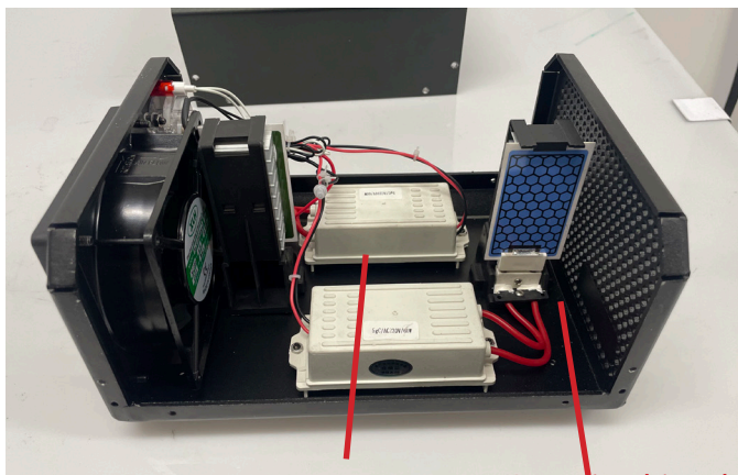
Otsonilevy
