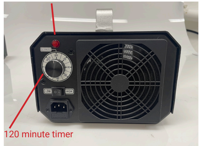
Indicator lamp
