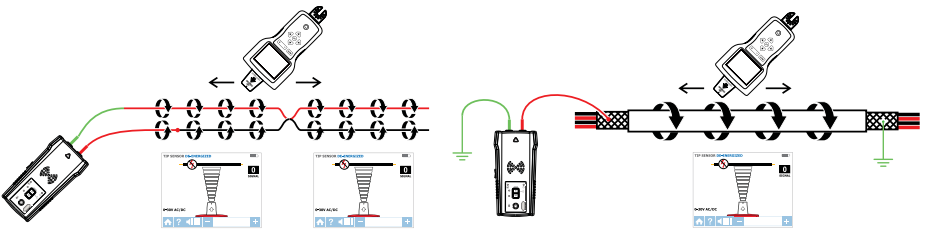
Figure 2.2a: Generating a signal with HIGH and LOW modes and closed loop Loop mode generates a signal (current flow) in closed loop De-energized circuits only. Loop mode is used to pinpoint the location of a short (because the current will not be able to flow in open branches) and to trace wires that are grounded on the far end (because the loop is closed via ground connection).
