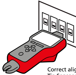
Correct alignment of the Tip Sensor to the breaker/fuse
